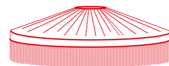
ABS6 diam.60x10x h.30cm ABS8 diam.80x20x h.30cm ABS10 diam.100x20x h.30cm ABS12 diam.120x30x h.30cm
